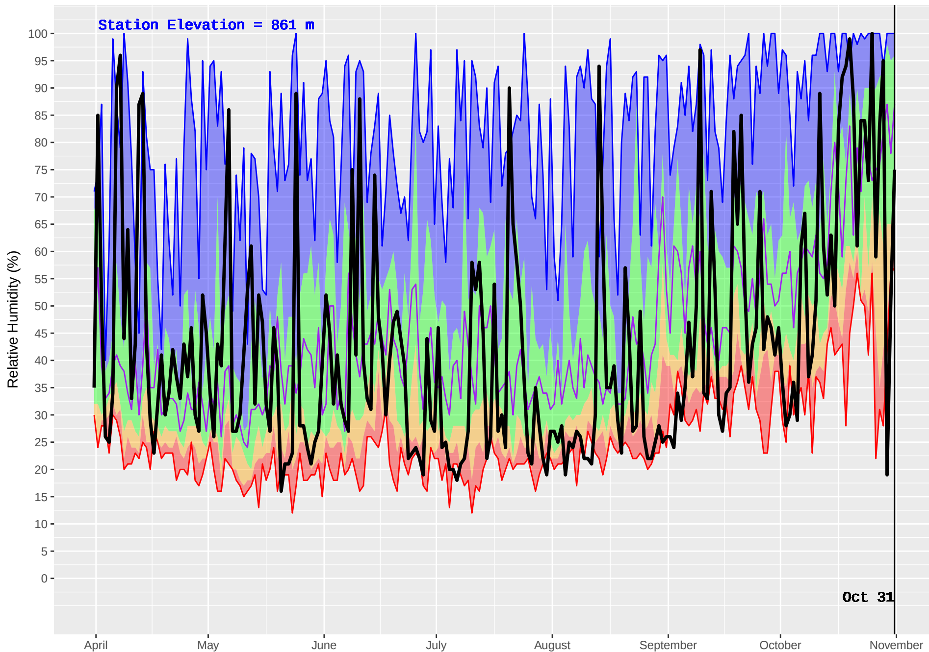
BLAEBERRY (866) : Historical (2004–2016) and Current (2017) Noon Relative Humidity
