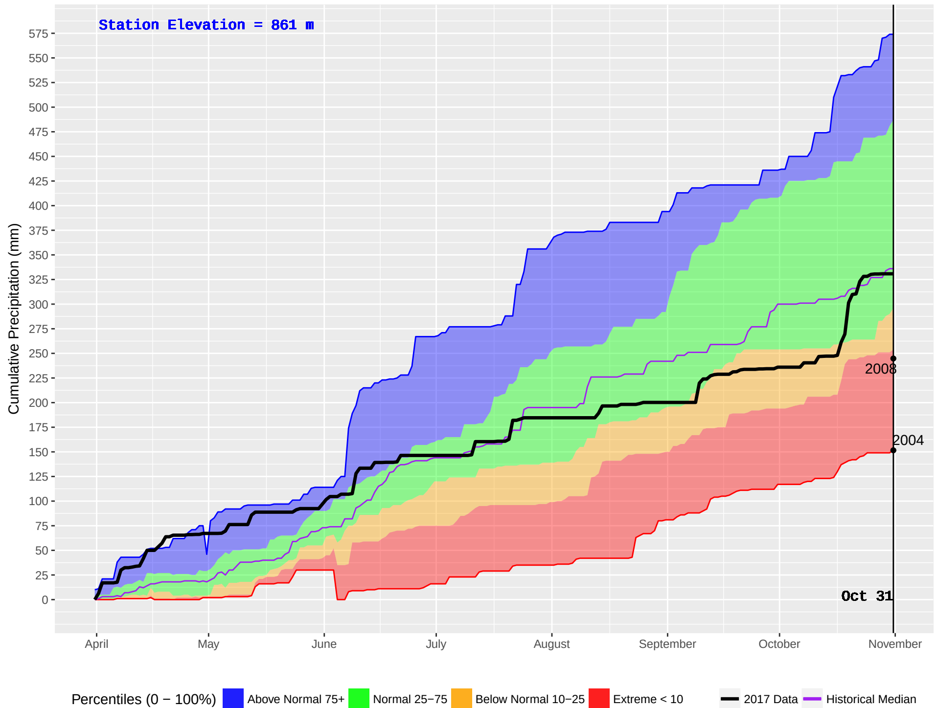
BLAEBERRY (866) : Historical (2004–2016) and Current (2017) Noon Cumulative Precipitation
