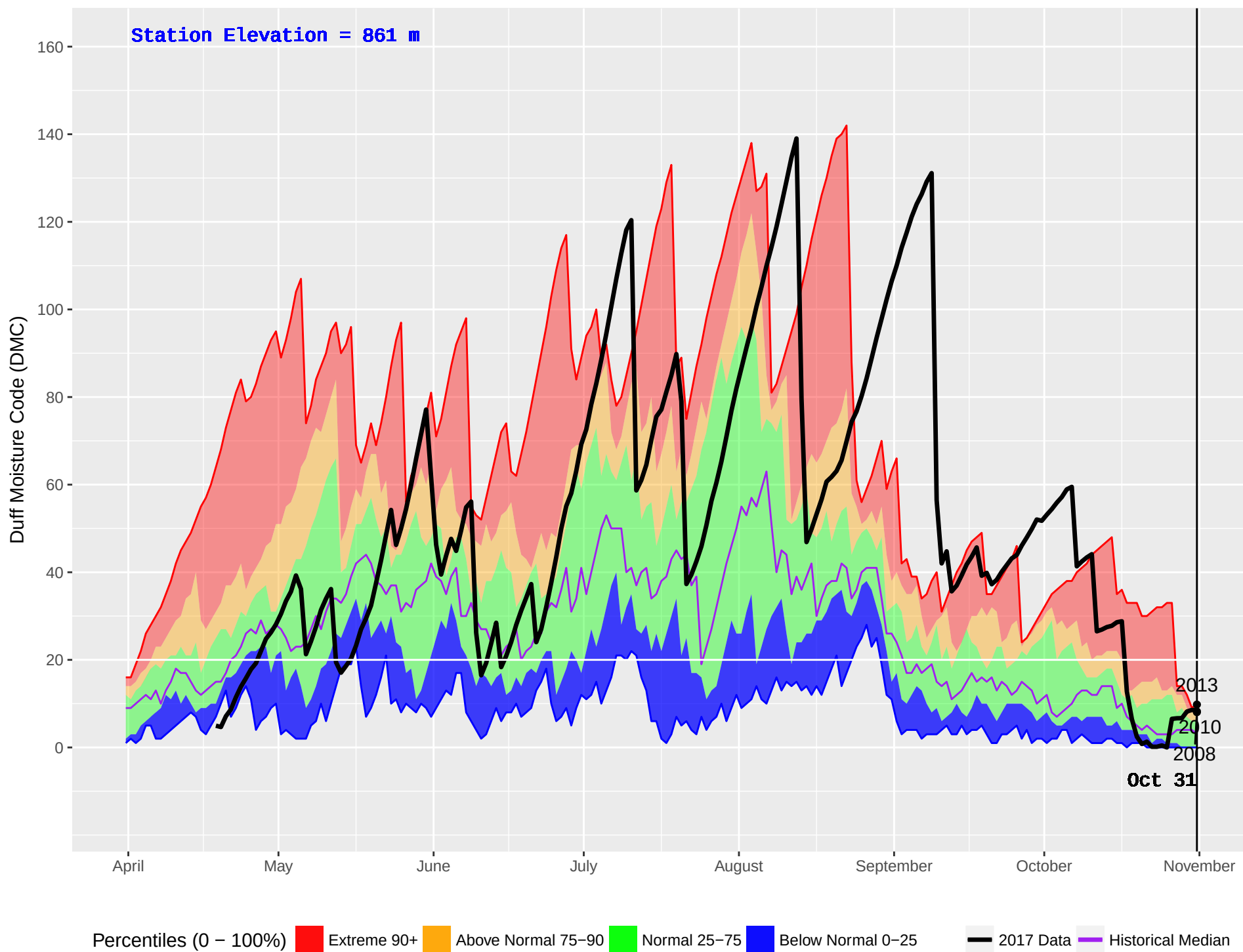
BLAEBERRY (866) : Historical (2004–2016) and Current (2017) Noon Duff Moisture Code (DMC)
